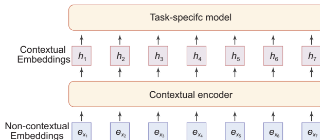
Figure 1 (Color online) Generic neural architecture for NLP.
