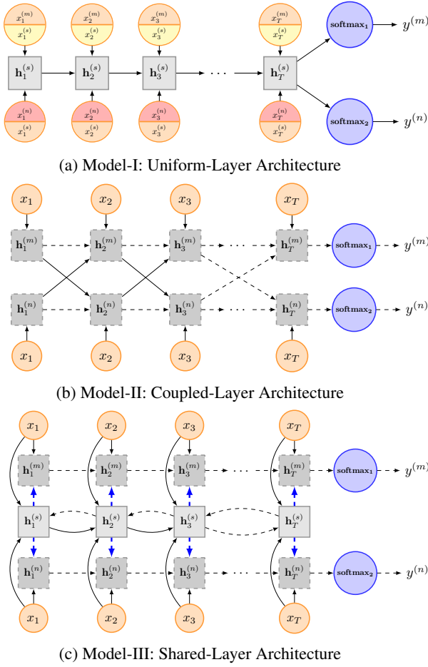
Figure 2: Three architectures for modelling text with multi-task learning.
